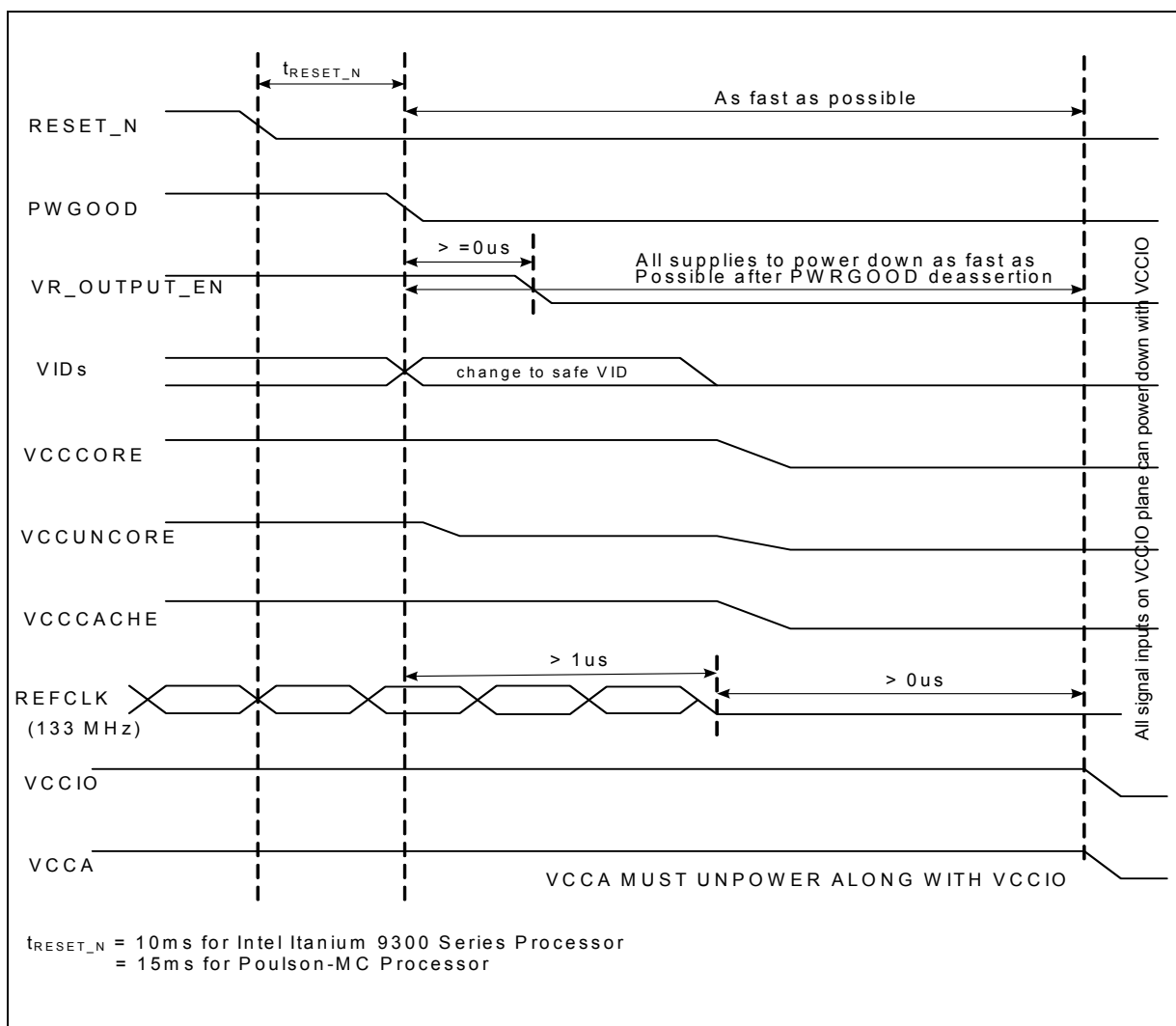
Figure 2-19. Supported Power-down Voltage Sequence Timing Requirements
