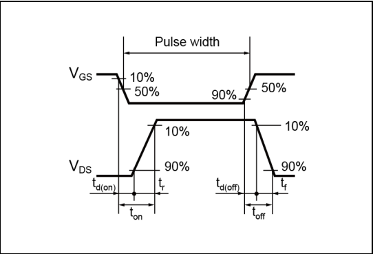
Fig.1-2 Switching Waveforms
