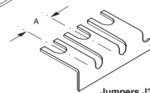
Jumpers J3
