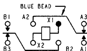
TERMINAL VIEW
