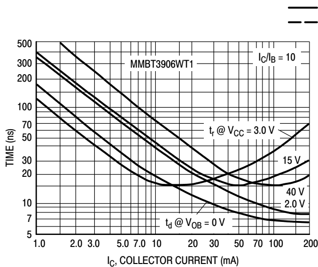
Figure 24. Turn-On Time
