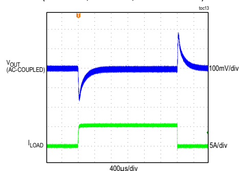
LOAD TRANSIENT RESPONSE (5V OUTPUT, PWM MODE, FIGURE 8 CIRCUIT)
