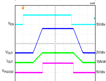
SOFT-START/SHUTDOWN FROM EN (5V OUTPUT, PWM MODE, FIGURE 8 CIRCUIT)
