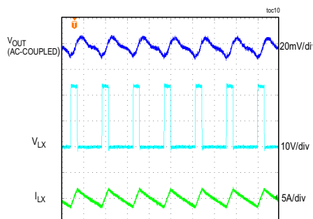
STEADY-STATE SWITCHING WAVEFORMS (5V OUTPUT, PWM MODE, FIGURE 8 CIRCUIT)
