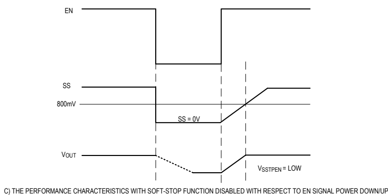
Figure 4. Soft-Stop Function Timing Diagram
