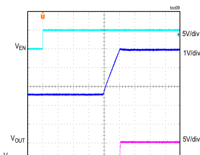
SOFT-START WITH 2.5V PREBIAS (5V OUTPUT, PWM MODE, FIGURE 8 CIRCUIT)
