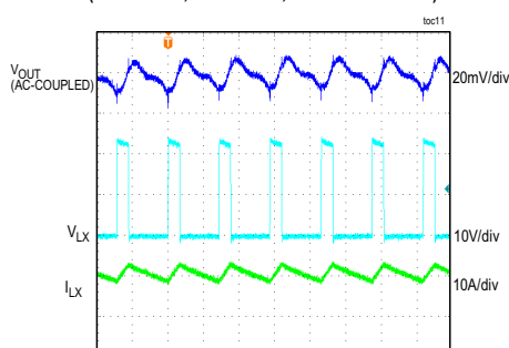
STEADY-STATE SWITCHING WAVEFORMS (5V OUTPUT, PWM MODE, FIGURE 8 CIRCUIT)
