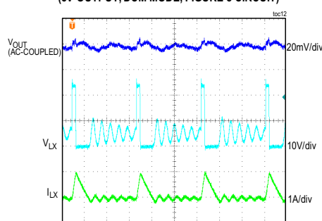
STEADY-STATE SWITCHING WAVEFORMS (5V OUTPUT, DCM MODE, FIGURE 8 CIRCUIT)
