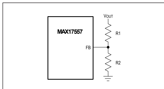
Figure 3. Output-Voltage Programming
