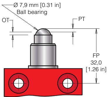
Figure 12. 24CE66 Dimensions
