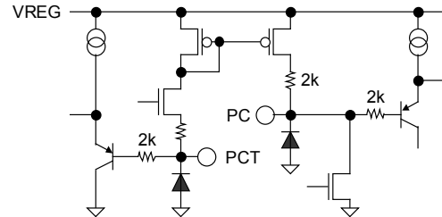
Figure 55. PC, PCT
