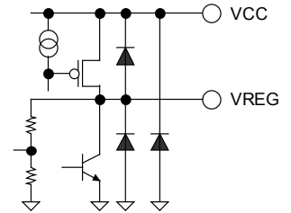
Figure 51. VREG, VCC
