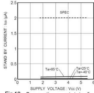
Fig.18 Consumption current at standby action ISB
