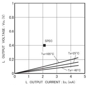
Fig.35 L output voltage VOL-IOL(Vcc=4.0V)
