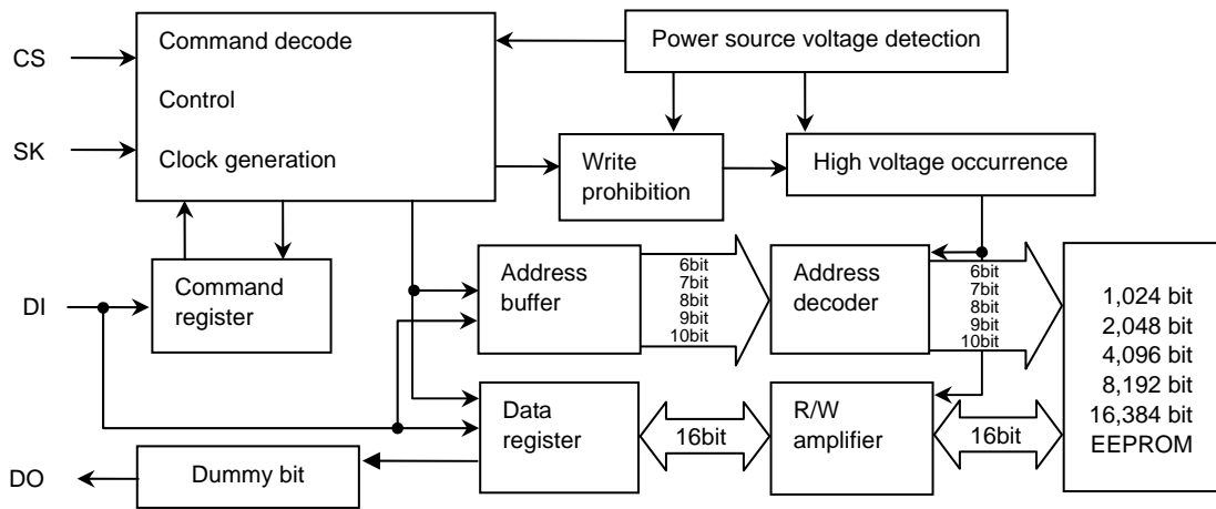
Fig.57 Block diagram
