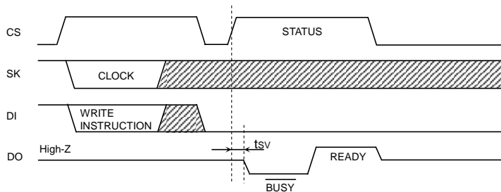
Fig.45 \text{R}/\overline{\text{B}} status output timing chart
