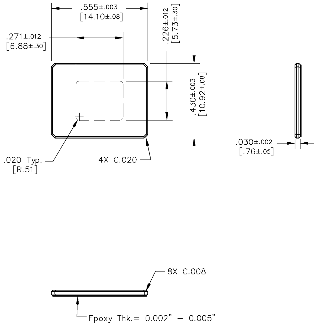
Figure 23: Glass Drawing
