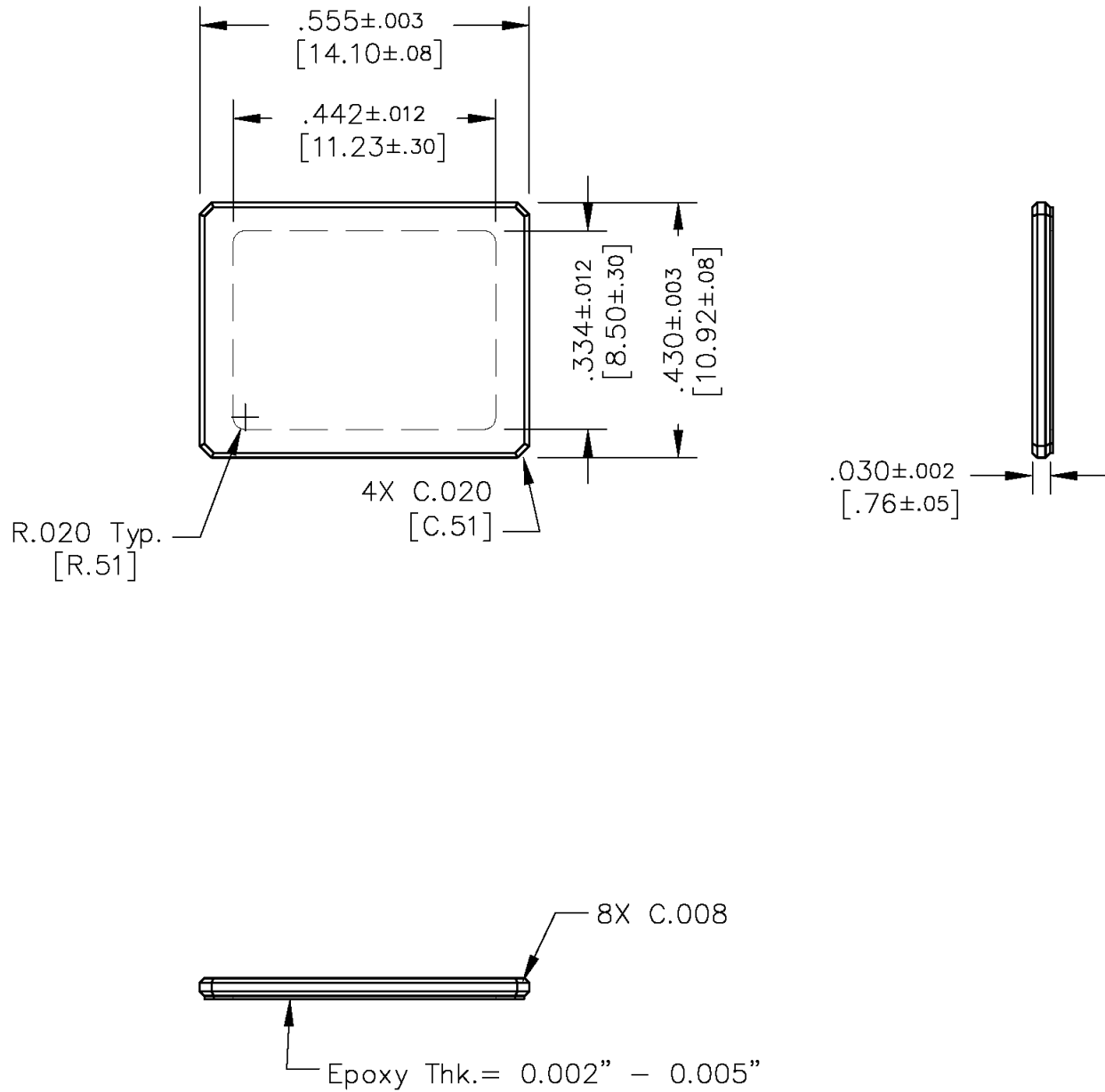
Figure 24: Quartz Cover Glass
