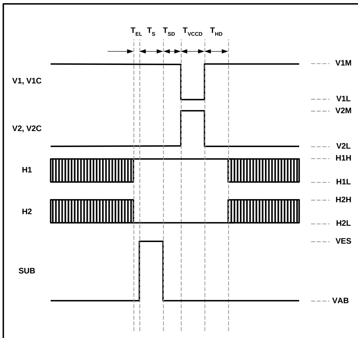
Figure 18: Electronic Shutter Timing
