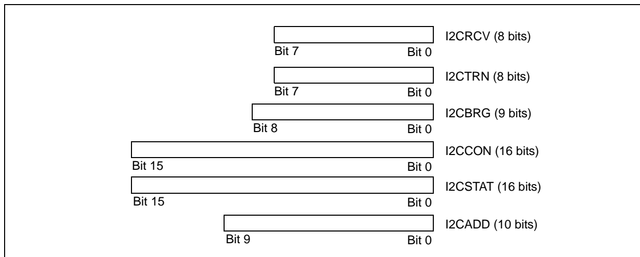
FIGURE 14-1: PROGRAMMER'S MODEL
