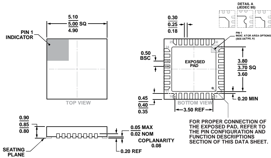
Figure 18. 32-Lead Lead Frame Chip Scale Package [LFCSP] 5 mm × 5 mm Body and 0.85 mm Package Height (HCP-32-1) Dimensions shown in millimeters
