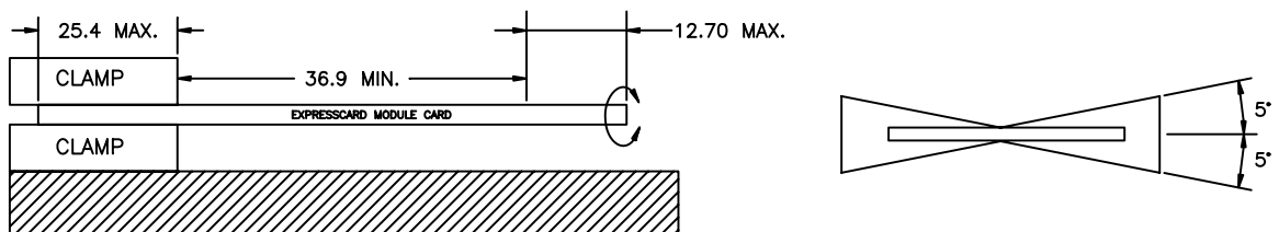
Figure for Torque Test
