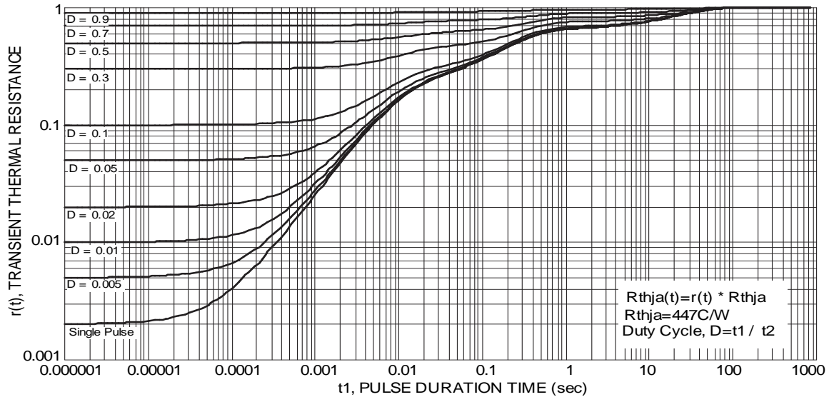
Figure 12 Transient Thermal Resistance
