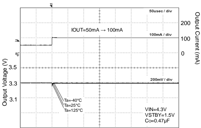
Figure 21. Load Response
