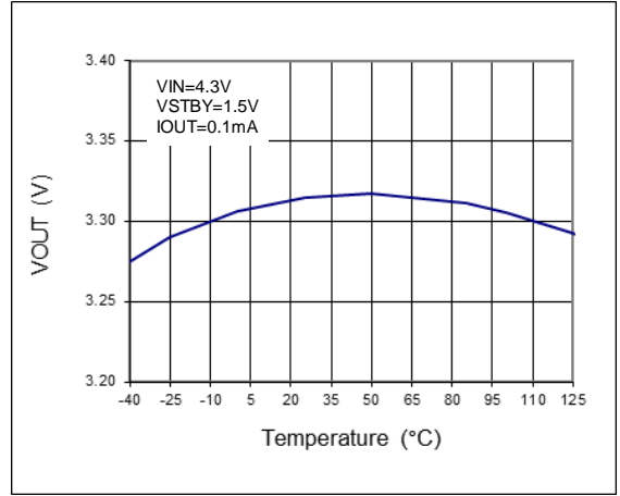
Figure 12. VOUT - Temp
