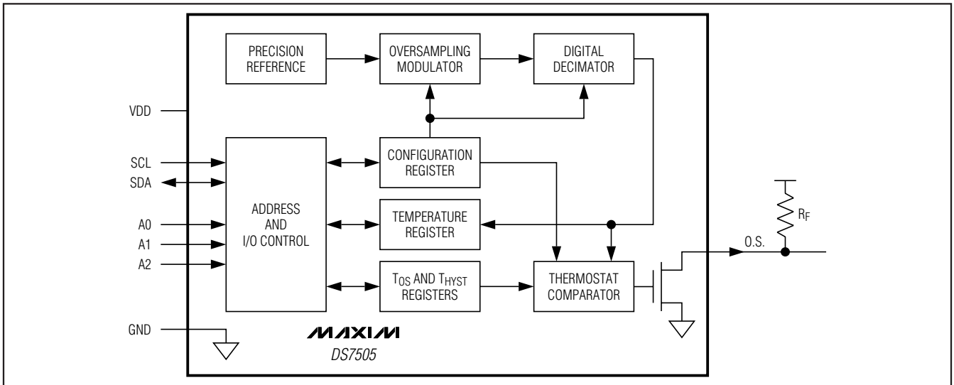
Figure 2. Block Diagram
