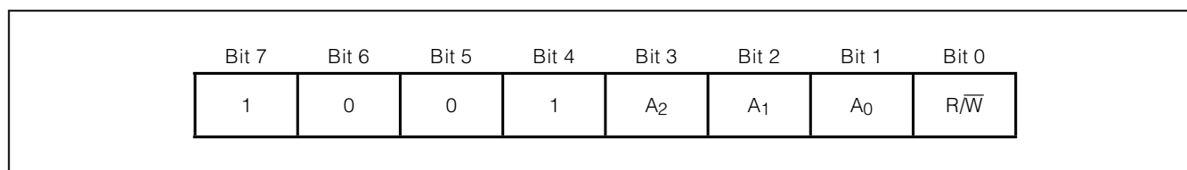
Figure 7. Address Byte
