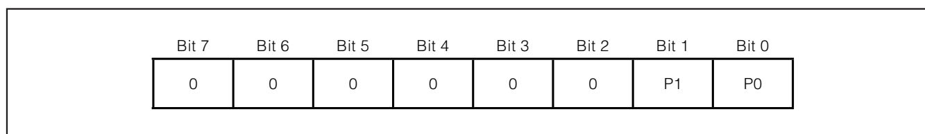
Figure 8. Pointer Byte
