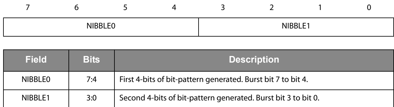
Figure 45: RAM Registers
