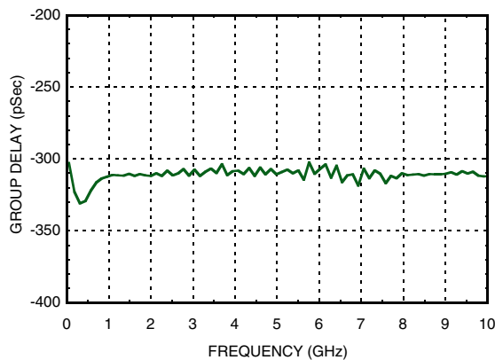
Group Delay
