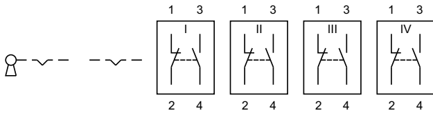
54 Keylock switch 2 positions page 11 | Keylock switch actuator 2 positions, flush mounting page 15
