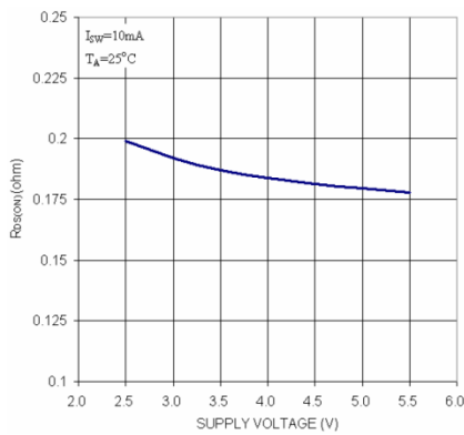
Fig. 12: PMOS R DS(ON) vs Supply Voltage
