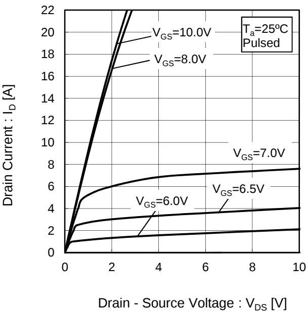
Fig.7 Typical Output Characteristics(II)
