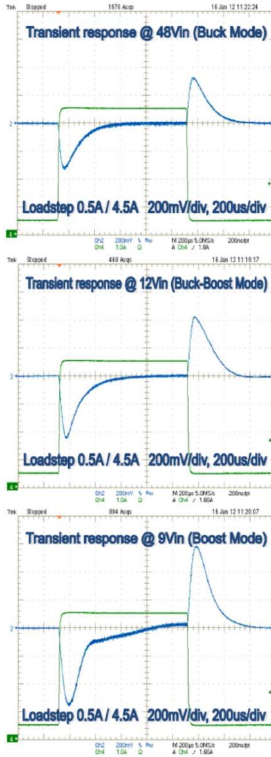
Figure 5. Load Transient Response
