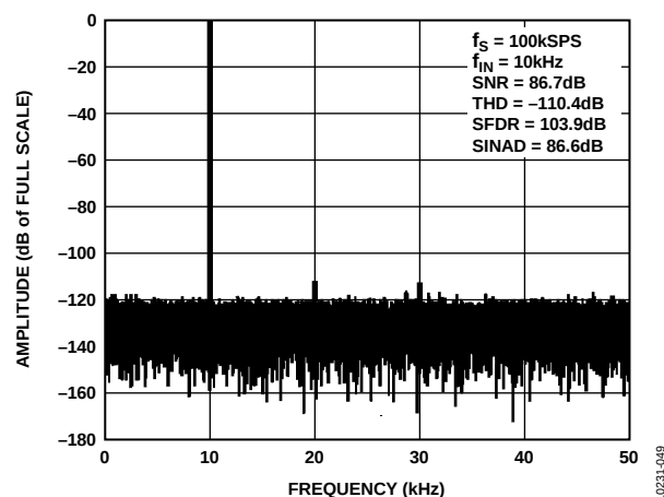
Figure 9. AD7988-1 FFT Plot, V REF = 2.5 V
