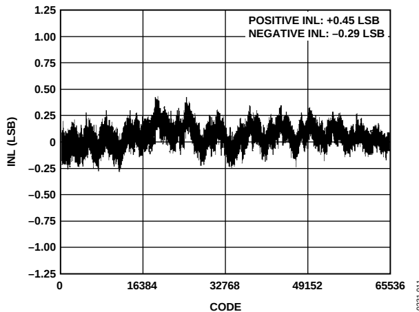
Figure 11. Integral Nonlinearity vs. Code, V REF = 2.5 V
