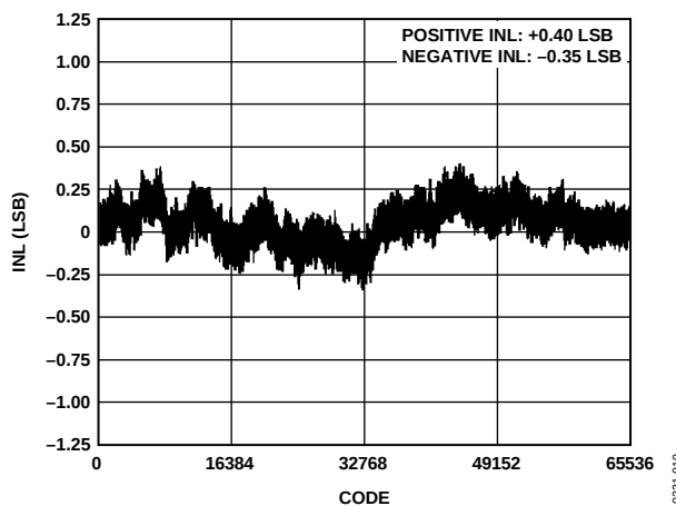
Figure 10. Integral Nonlinearity vs. Code, V REF = 5 V
