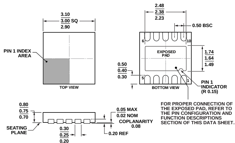
Figure 45. 10-Lead Lead Frame Chip Scale Package [QFN (LFCSP_WD)] 3 mm × 3 mm Body, Very Very Thin, Dual Lead (CP-10-9)
