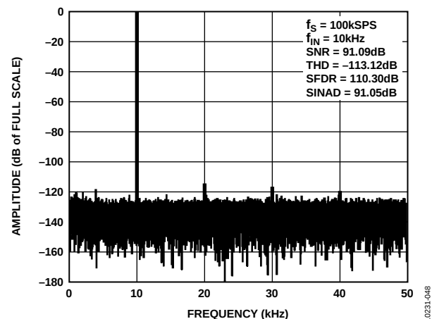
Figure 8. AD7988-1 FFT Plot, V REF = 5 V
