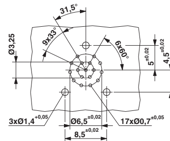
Drilling diagram
