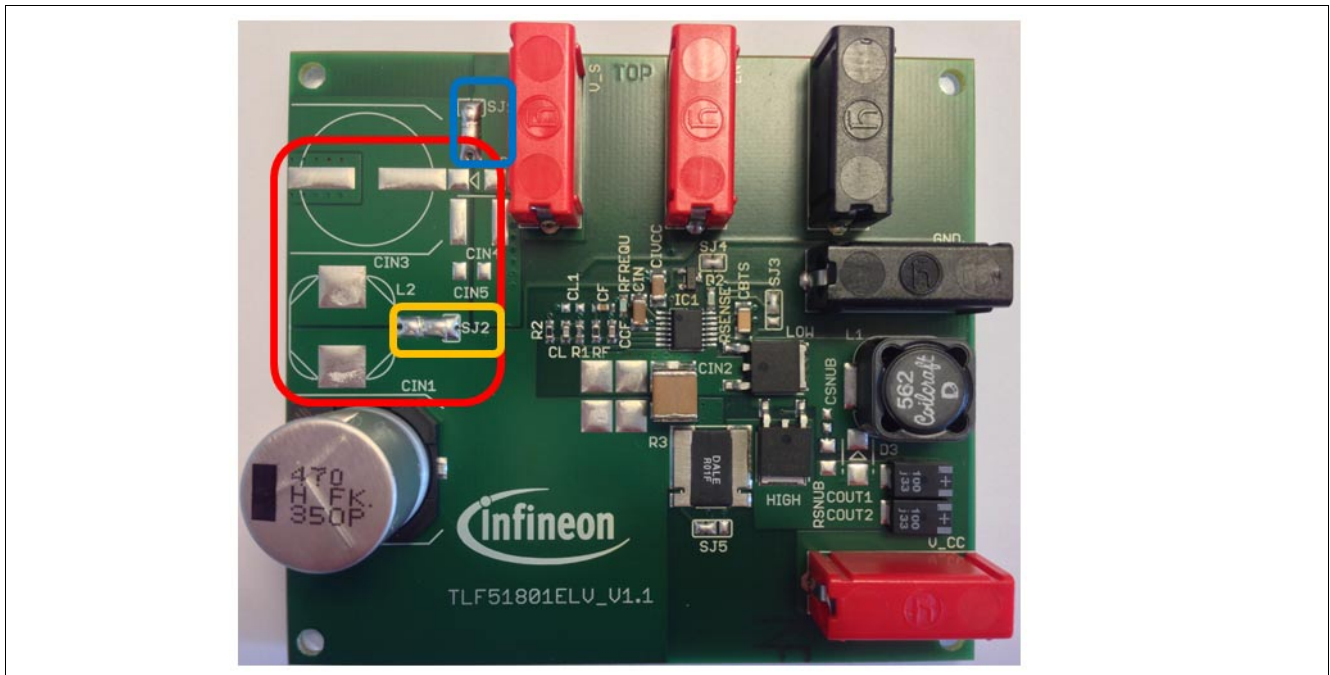
Figure 7 Input filter
