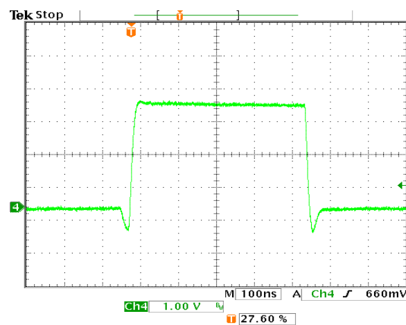
Figure 15. Switching Node Waveform at Auto CCM/DCM Mode V_{in} = 3.3\text{ V} , Full Load
