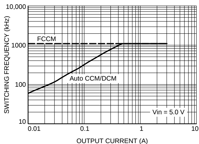
Figure 11. Switching Frequency vs. Output Current at V_{in} = 5.0\text{ V}
