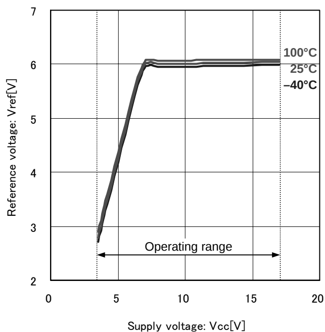
Fig.16 Reference voltage
