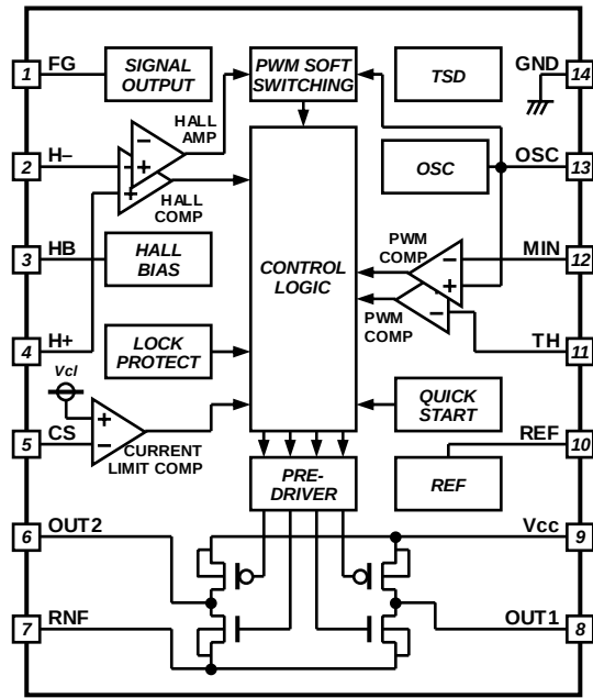
Fig.2 Block diagram
