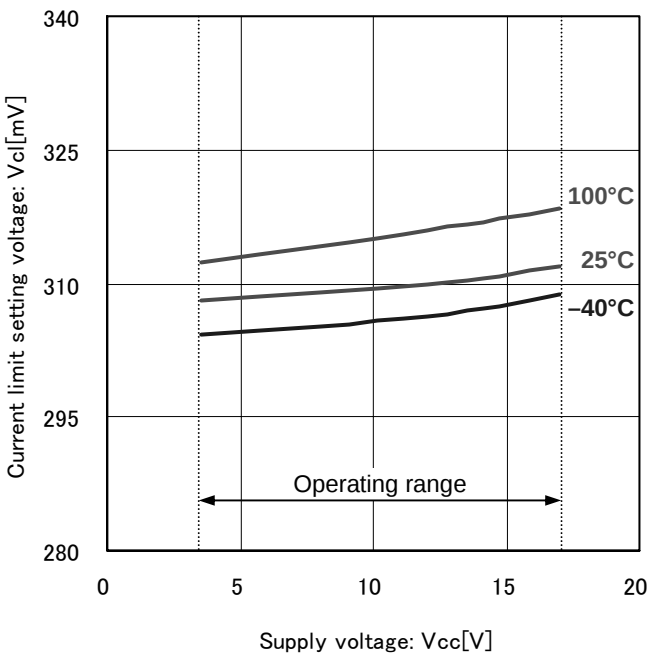
Fig.20 Current limit setting voltage
