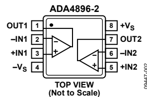
Figure 5. 8-Lead MSOP Pin Configuration
