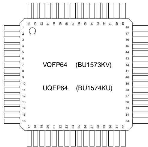
(BU1573KV/BU1574KU Top View)
