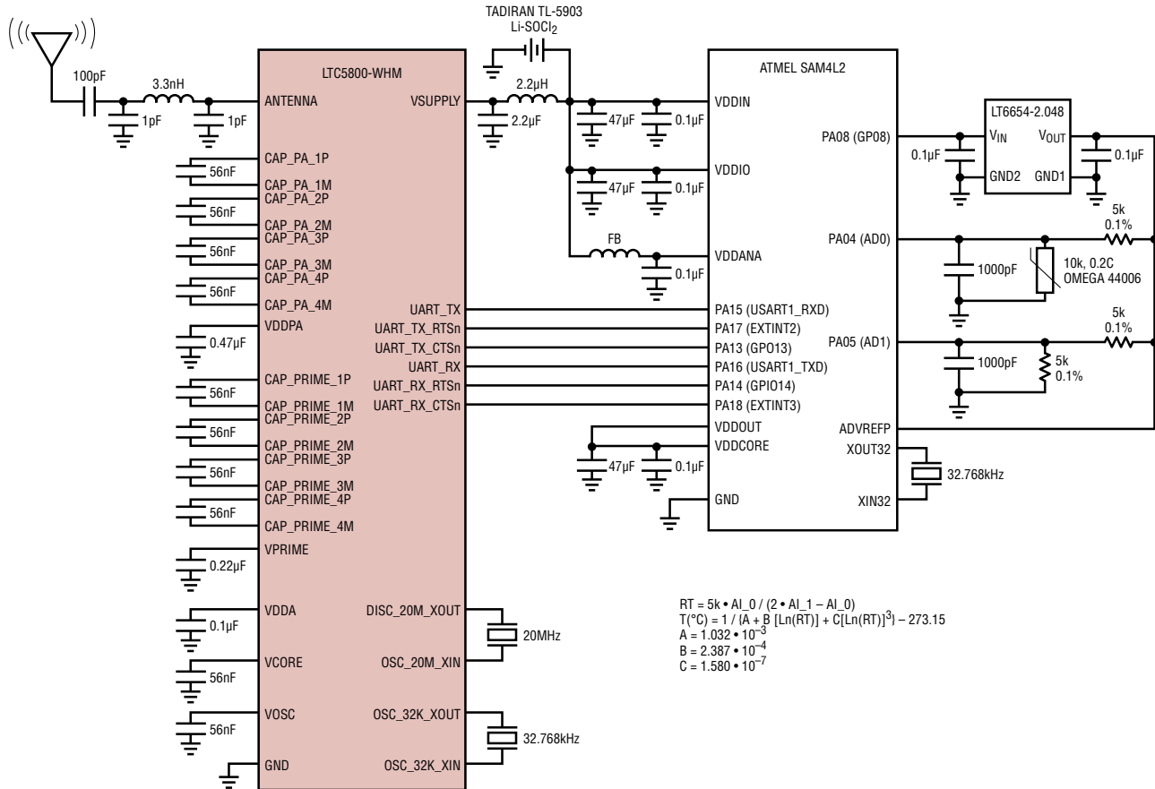
Mesh Network Thermistor
