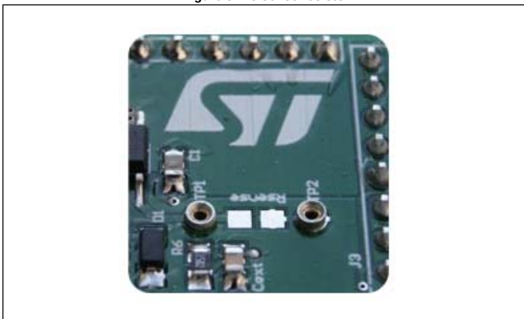
Figure 4. Mounting through-hole sense resistor
