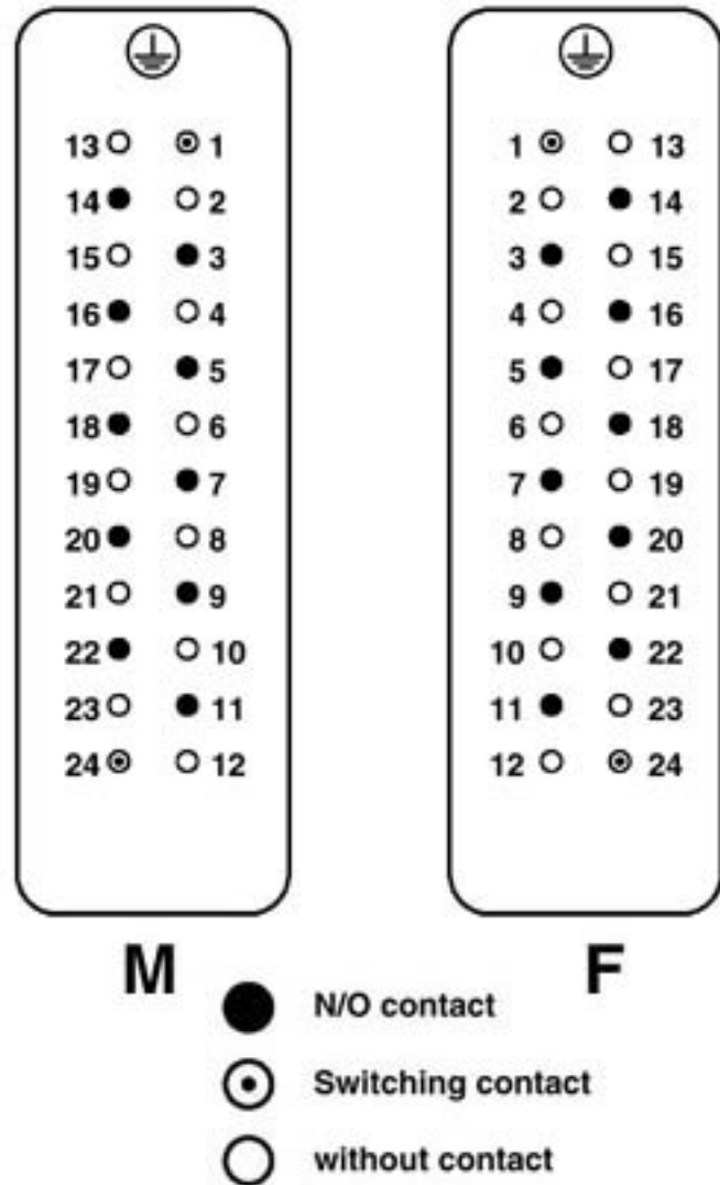
View termination side
