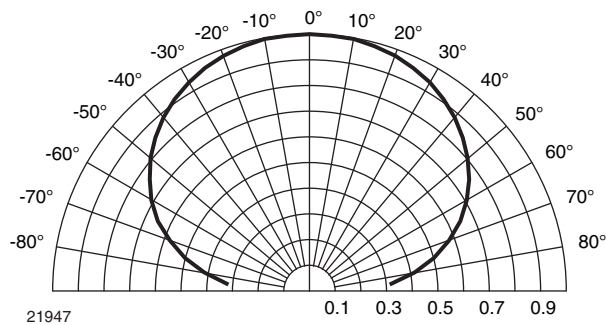
Fig. 11 - Horizontal Directivity
