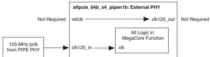
Figure 3–29. Generic PIPE PHY Clock Configuration (1)
