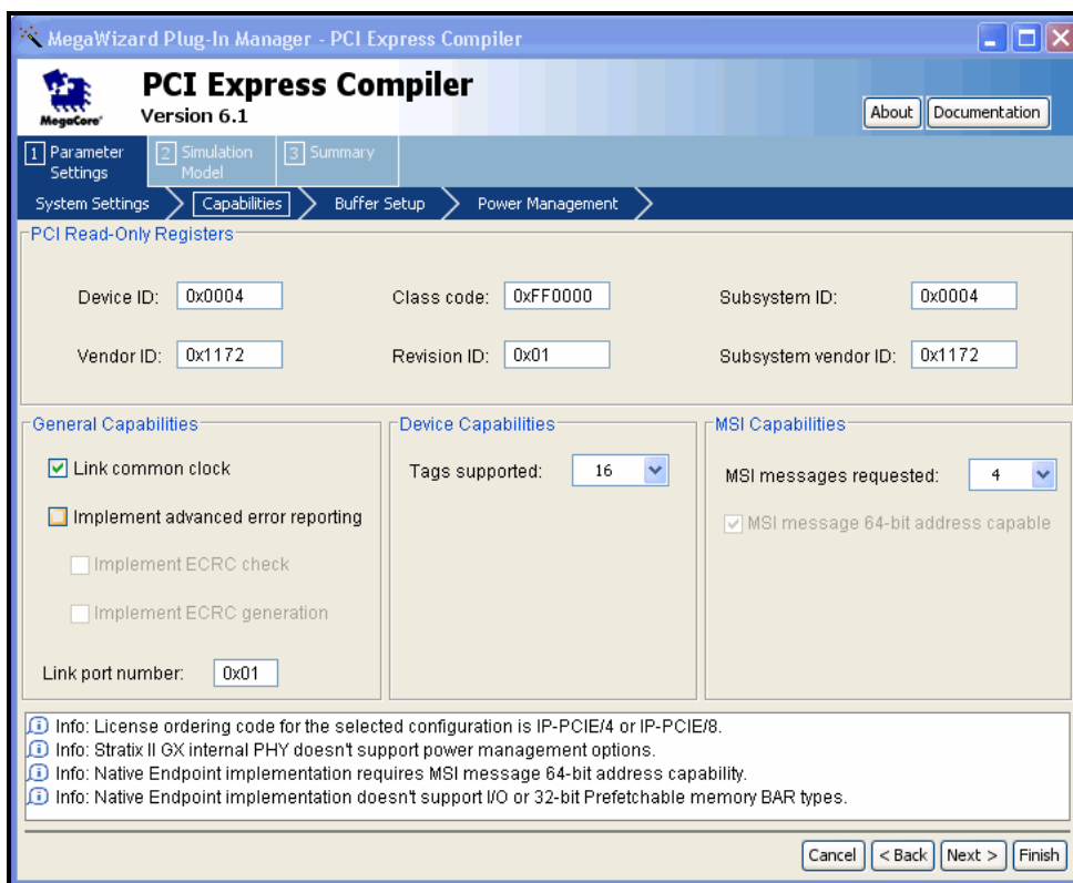
Figure 2–5. Capabilities Page
