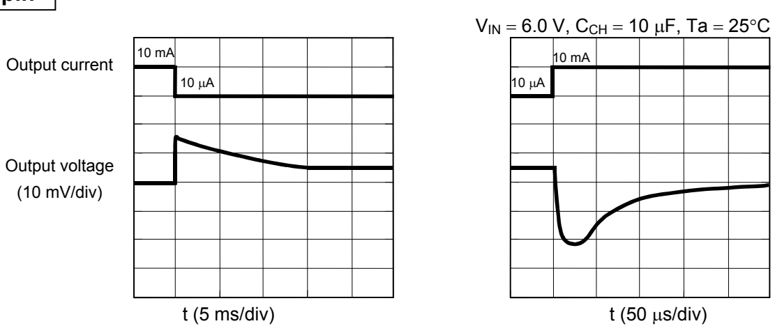
Figure 24 Ringing Waveform due to Load Variation (VCH Pin)
