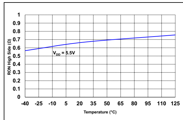
FIGURE 2-6: Outputs R_{ON} High-Side Resistance vs. Temperature.
