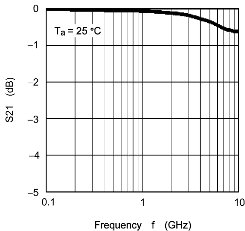
Fig. 9.5 S_{21} - f
