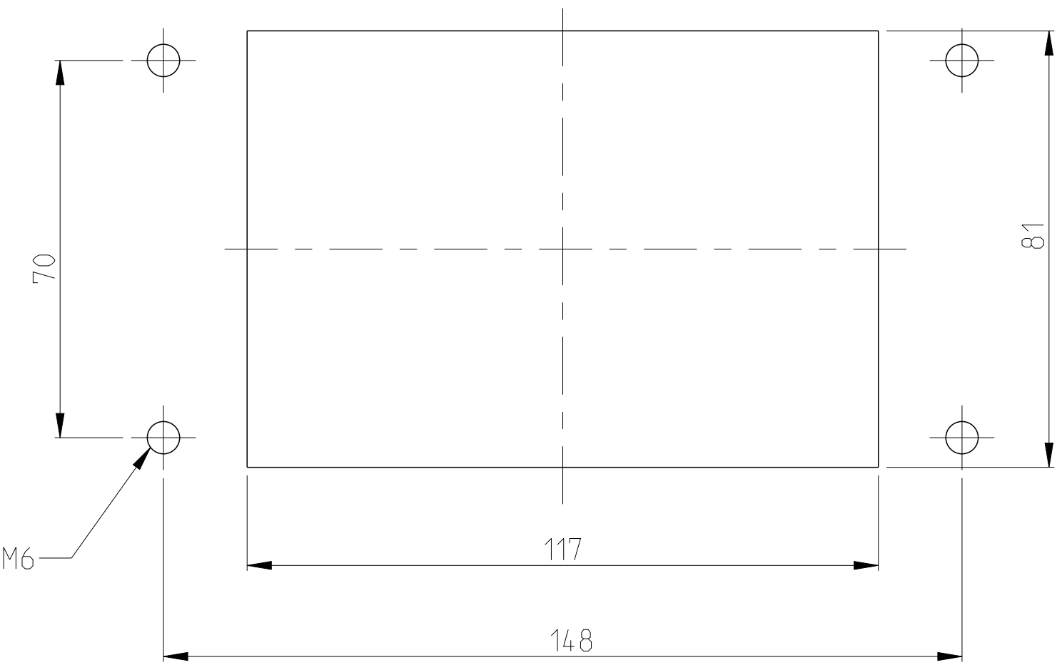
PANEL CUT-OUT
