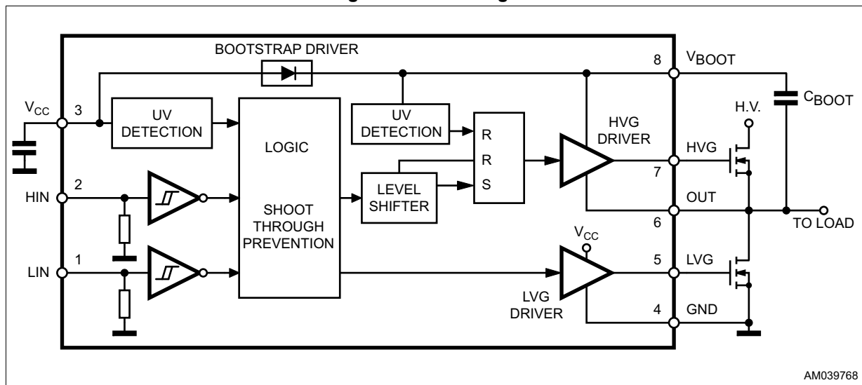
Figure 1. Block diagram
