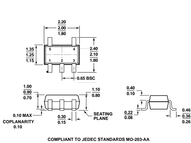
Figure 38. 5-Lead Thin Shrink Small Outline Transistor Package [SC-70] (KS-5) Dimensions shown in millimeters
