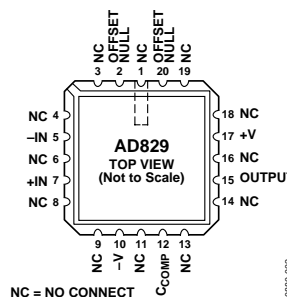
Figure 2. 20-Terminal LCC
