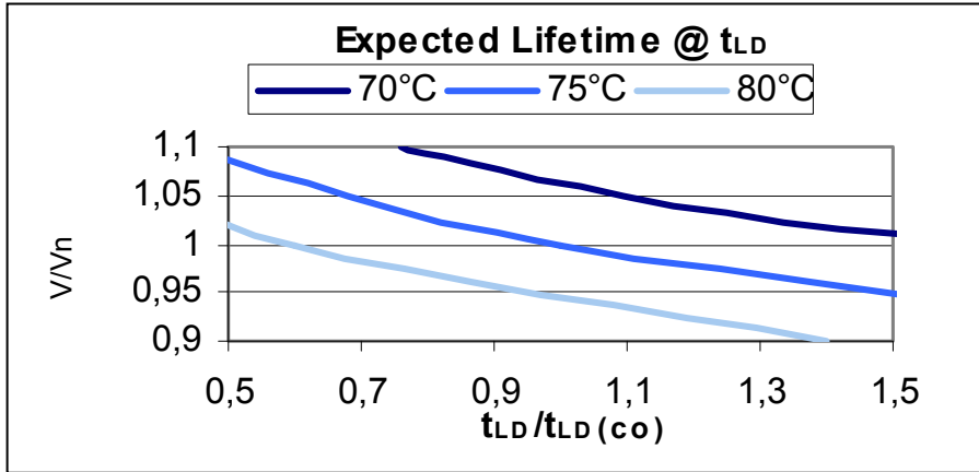
Expected lifetime t_{ld} at different hotspot temperature ( \Theta_{hs} ) and voltage V
