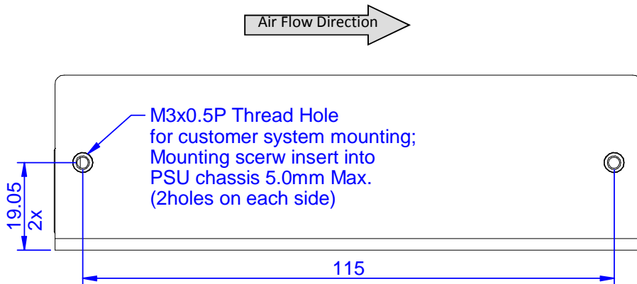
Figure 19: Side view 1
