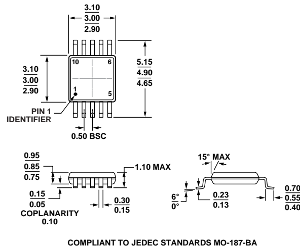
Figure 44. 10-Lead Mini Small Outline Package [MSOP] (RM-10) Dimensions shown in millimeters
