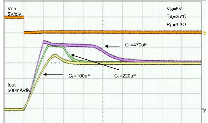
Inrush Current
