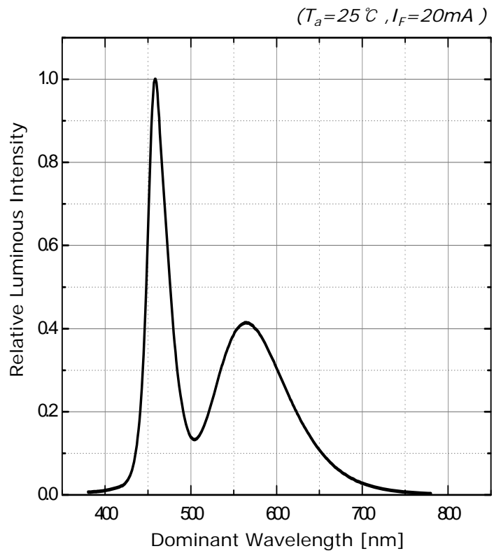
Spectral distribution
